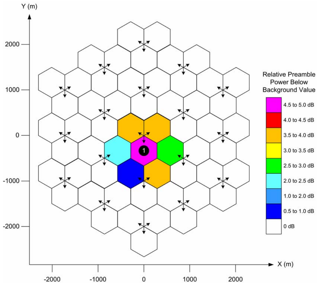
Figure 10 The average preamble power for the top ten configurations
