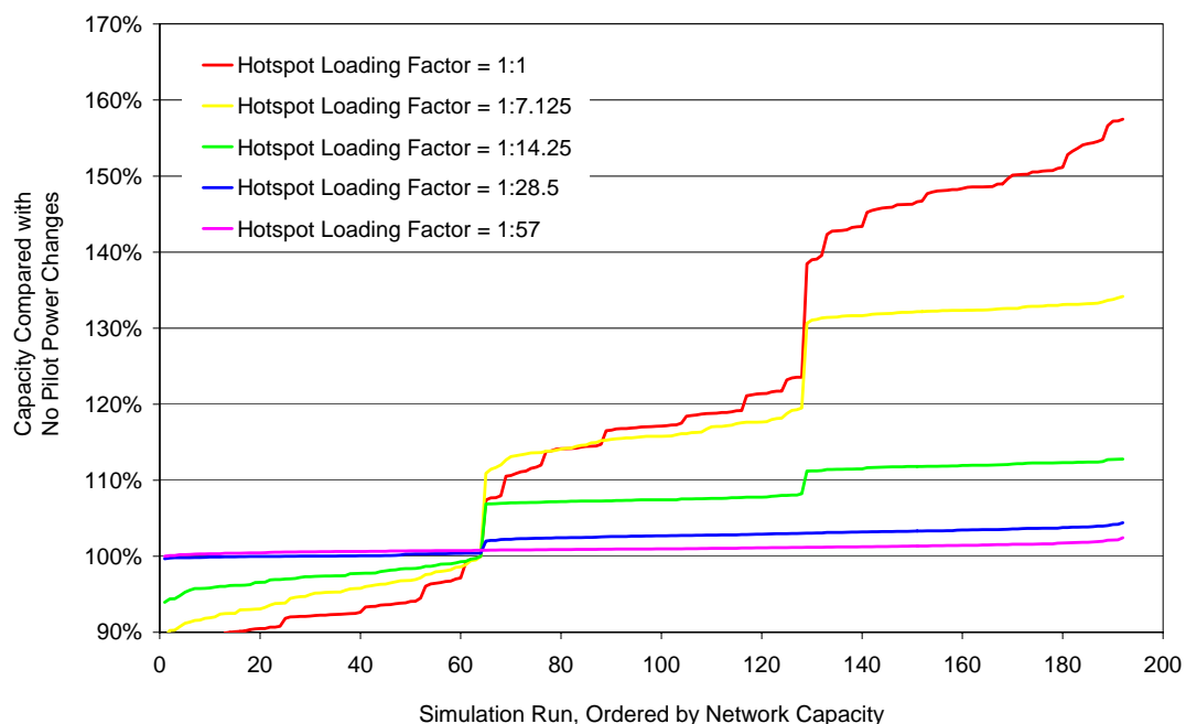
Figure 3 Uplink capacity gain for pilot power optimisation with an active set size of six
