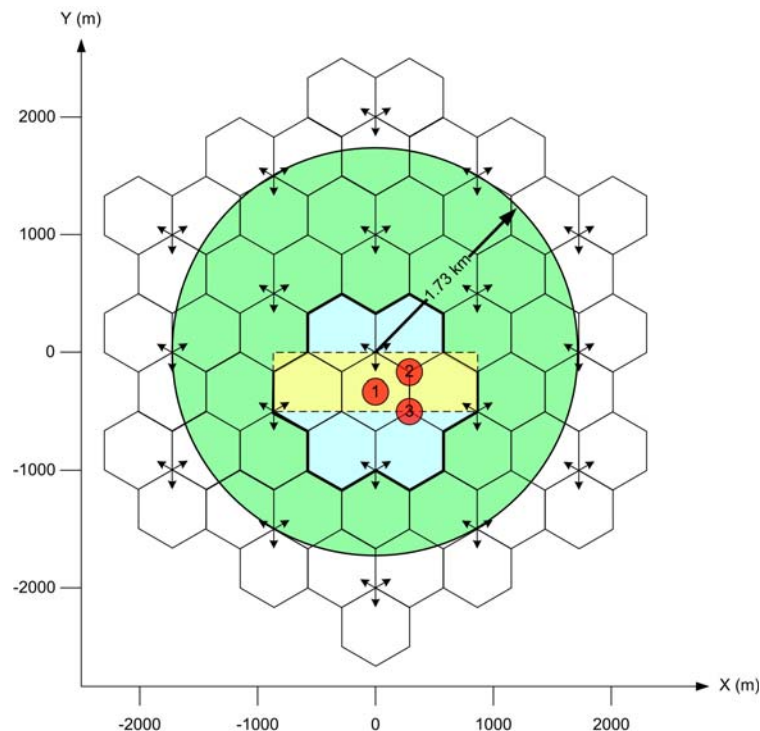
Figure 7 The 4G network used for the simulations
