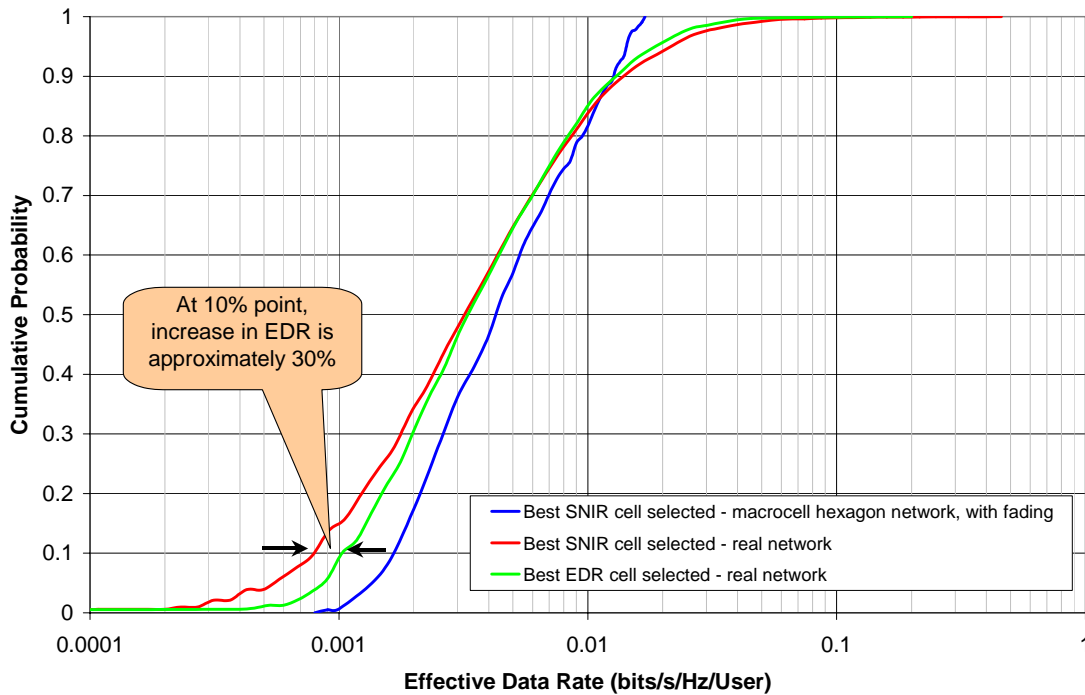
Figure 14 EDR distribution for a realistic user distribution in part of Vodafone's network using different cell selection methods
