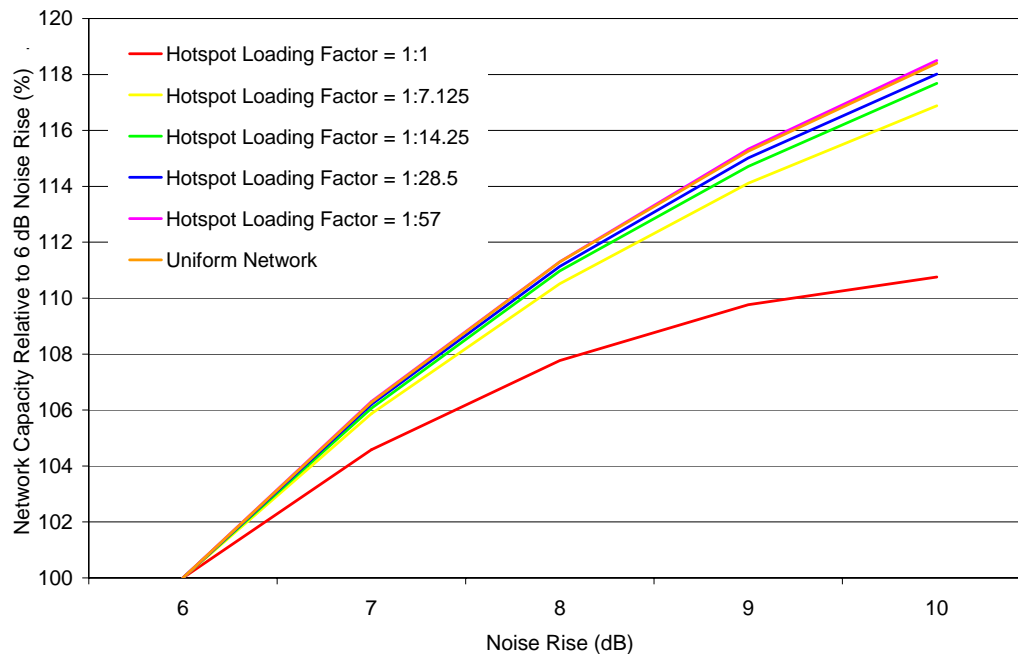
Figure 5 Capacity improvement as noise rise is increased
