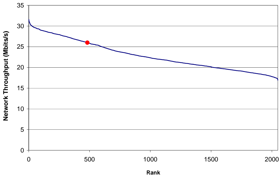
Figure 9 Simulation result for Hotspot 1 with a 25% weighting
