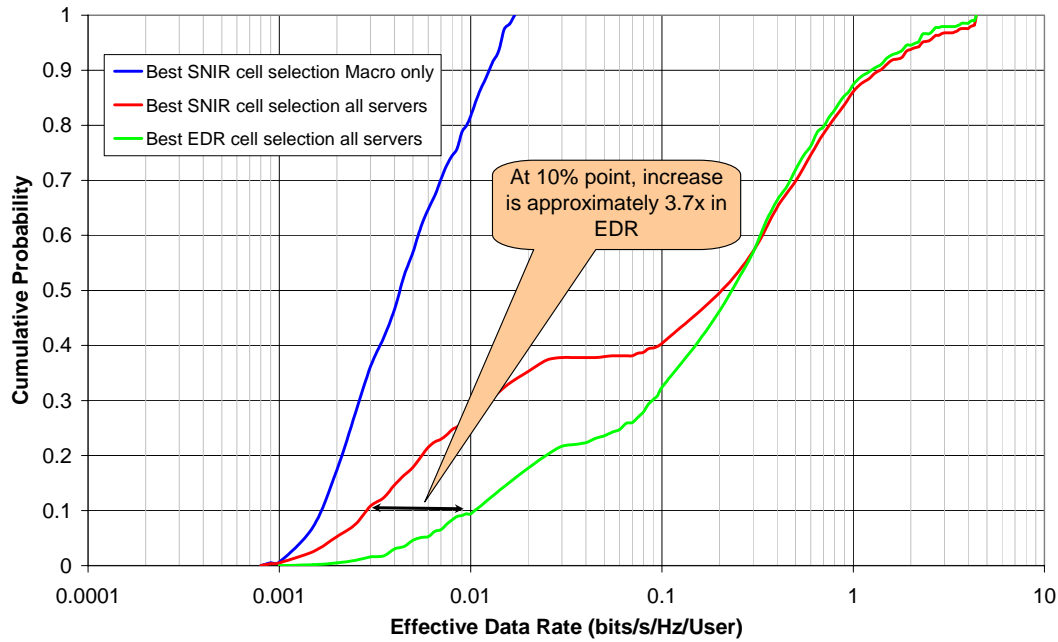
Figure 20 Downlink EDR distribution for users in a mixed macrocell and femtocell scenario using different cell selection methods across all users
