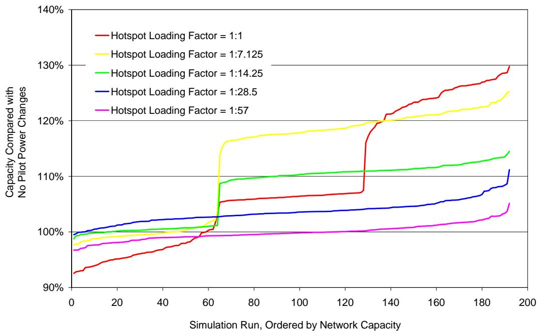
Figure 4 Downlink capacity gain for pilot power optimisation with an active set size of six
