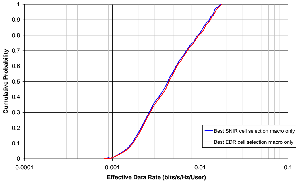
Figure 11 EDR distributions for users in a macrocell-only environment using different cell selection methods, distribution across all users
