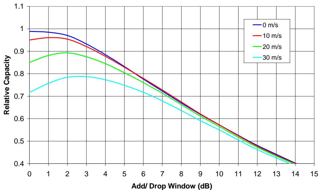
Figure 6 The relationship between network capacity and the handover add/drop window
