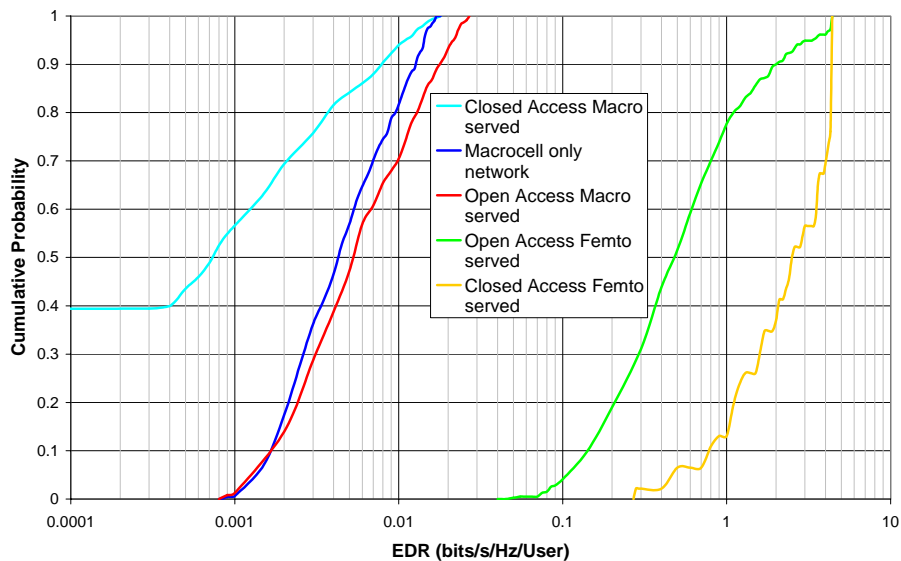
Figure 17 Downlink EDR distributions for Open and Closed Access configurations, with servers selected by the best SNIR
