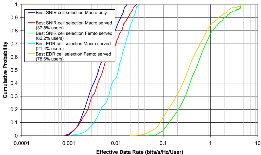
Figure 19 EDR distribution for users in a mixed macrocell and femtocell environment using different cell selection methods with the distributions categorised by server
