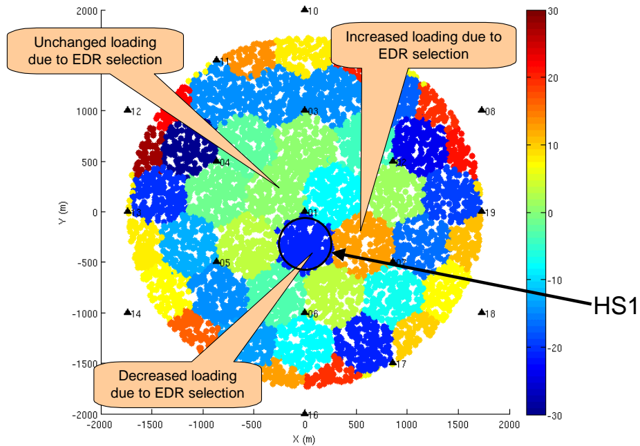
Figure 12 Difference in cell loading when moving from a Best SNIR to Best EDR cell selection scheme
