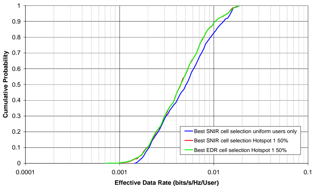
Figure 13 EDR distribution for Hotspot 1 inserted into a uniform macrocell network using different cell selection techniques
