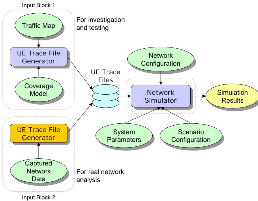
Figure 1 High level simulator design
