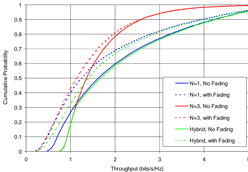
Figure 16 Cumulative distribution function of throughput for N=1 and N=3 reuse, along with a hybrid reuse scheme
