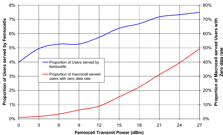
Figure 18 Performance characteristics for Closed Access femtocell operation as femtocell transmit power is varied
